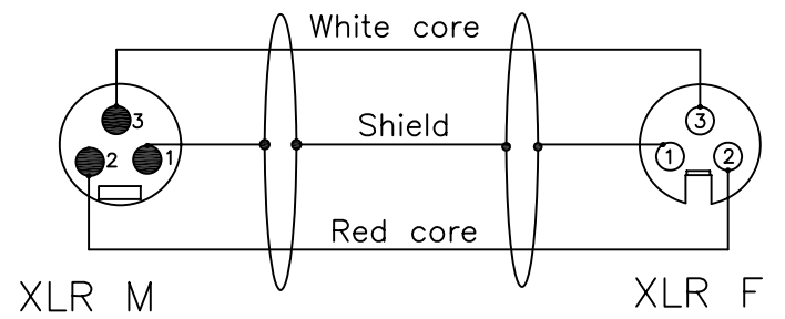
Wiring Method
